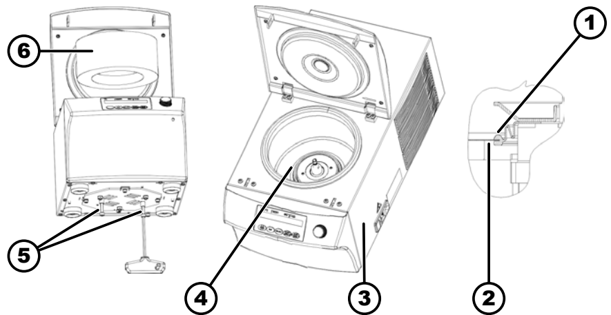
Fig. 14: Transport lock
